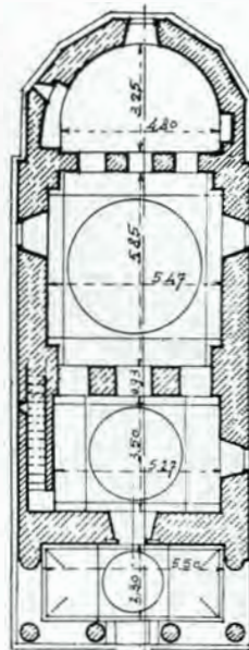
Fig. 280. — Plan
