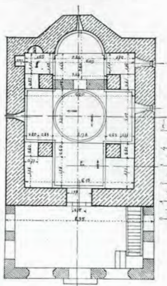
Fig. 102. — Plan
